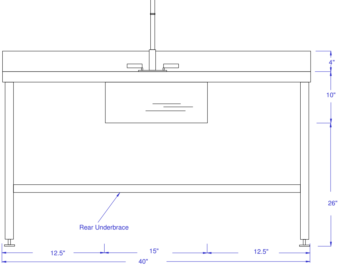
FRONT VIEW
